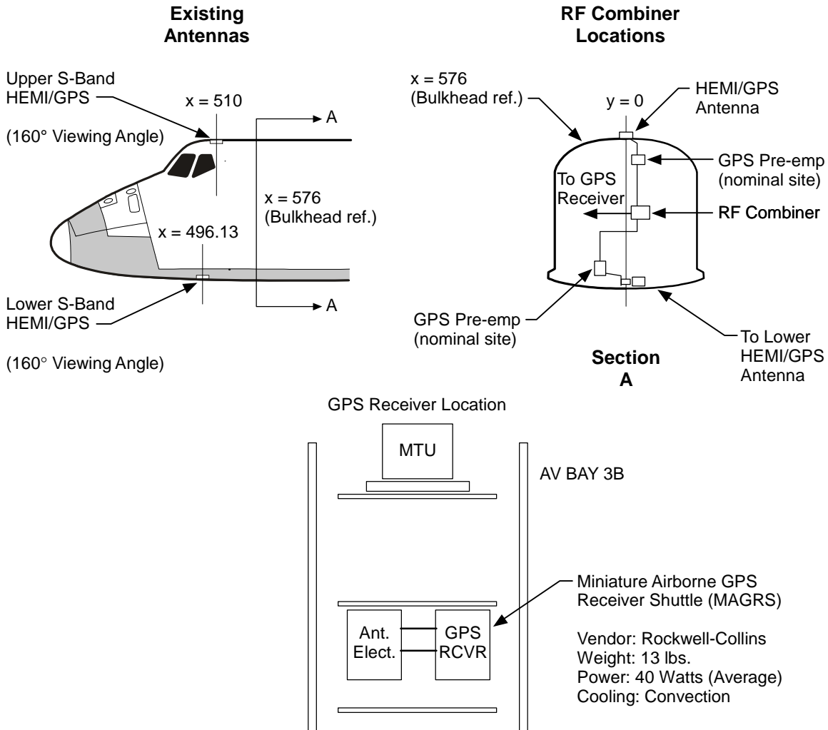
Figure 1-3. Single-string GPS antenna locations
