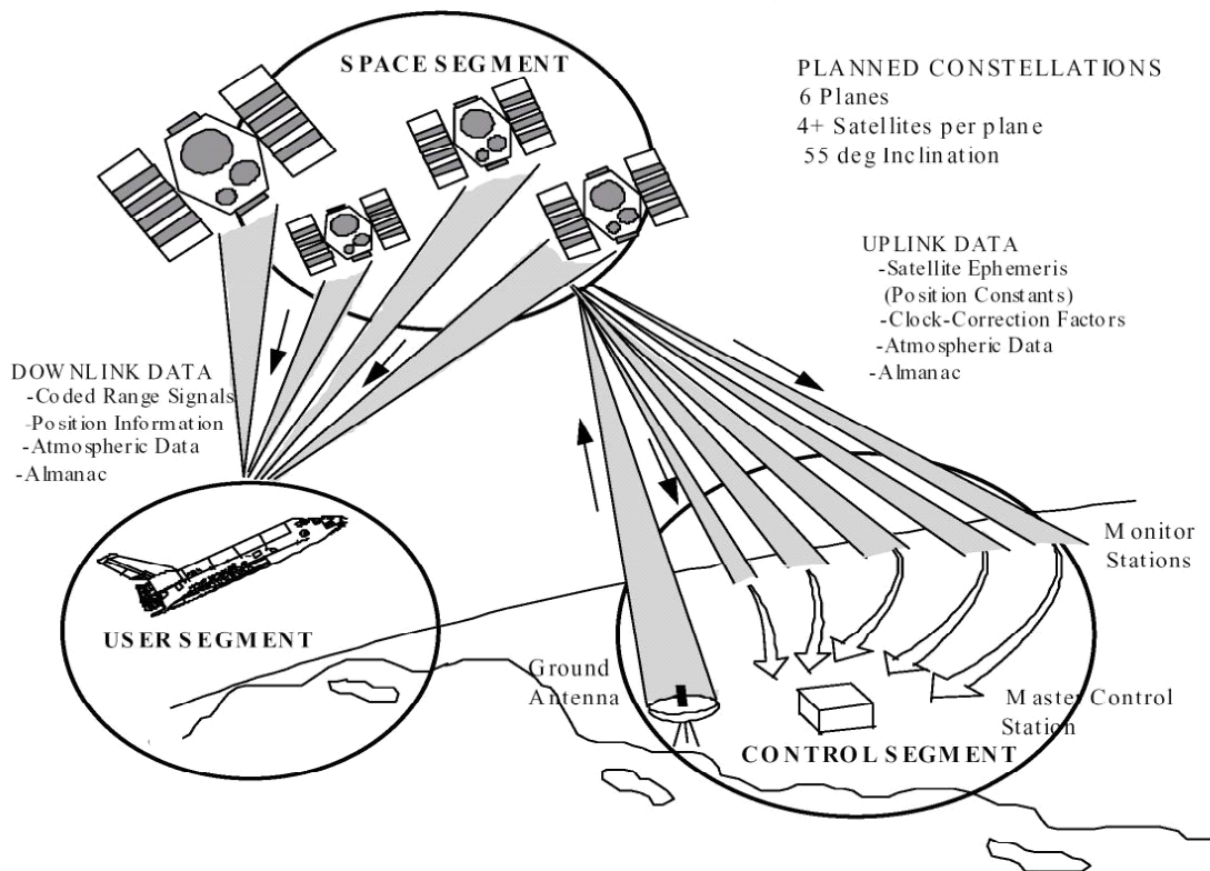
Figure 1-1. GPS overview
