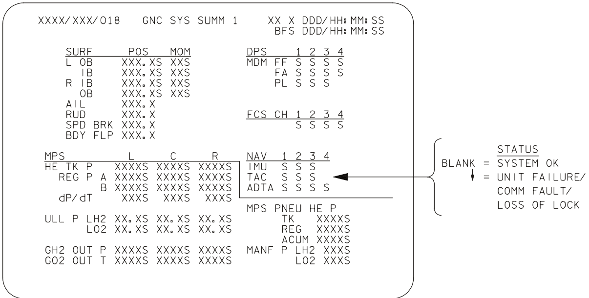
Figure 2-12. BFS GNC SYS SUMM 1 display
