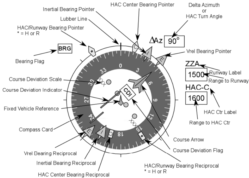
Figure 2-10. MEDS HSI
