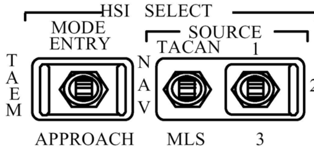
Figure 2-9. HSI switch location on Panels F6 and F8
