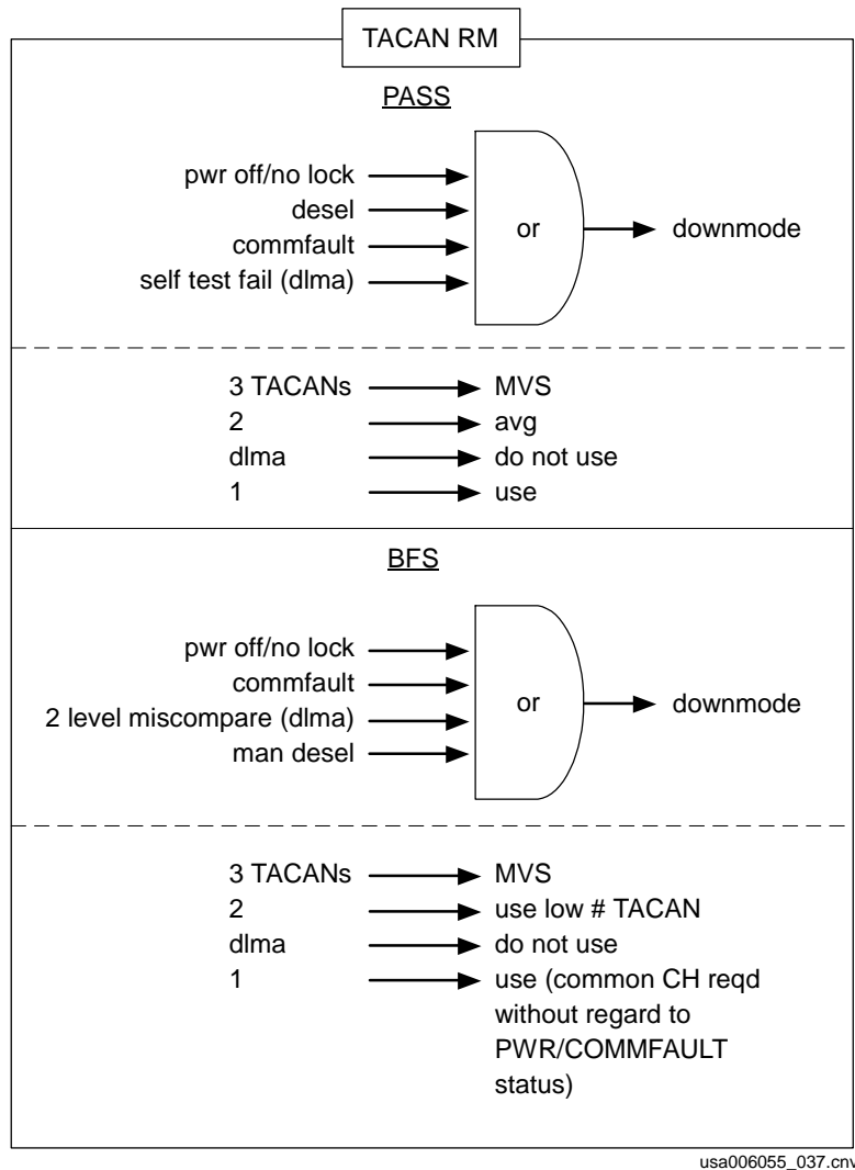
Figure 2-23. Entry pocket checklist TACAN RM summary
