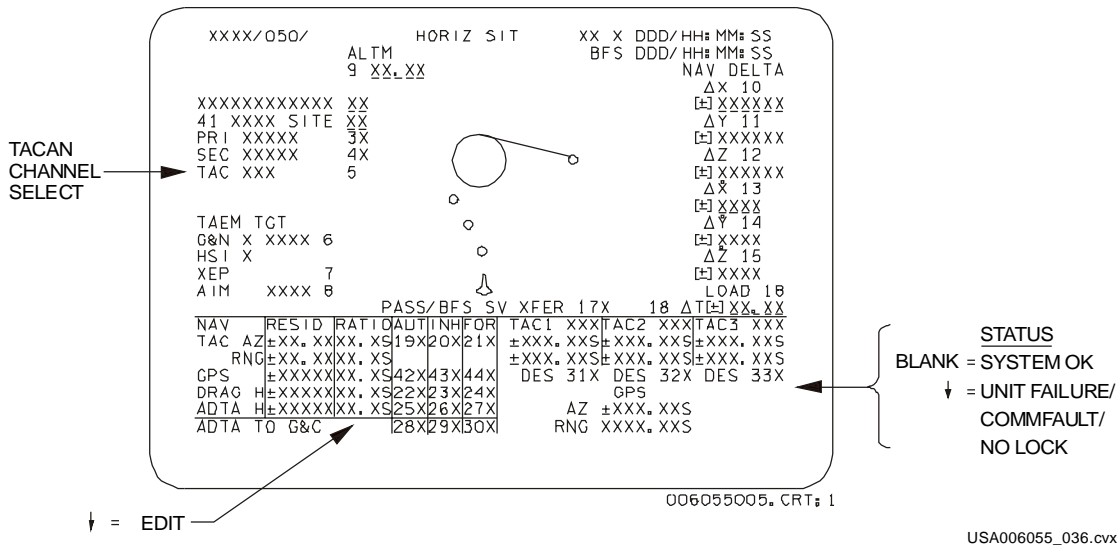
Figure 2-14. BFS GNC HORIZ SIT display
