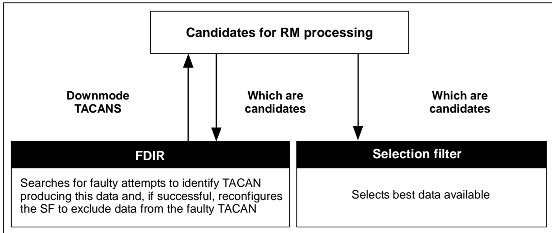
Figure 2-18. Redundancy management processing
