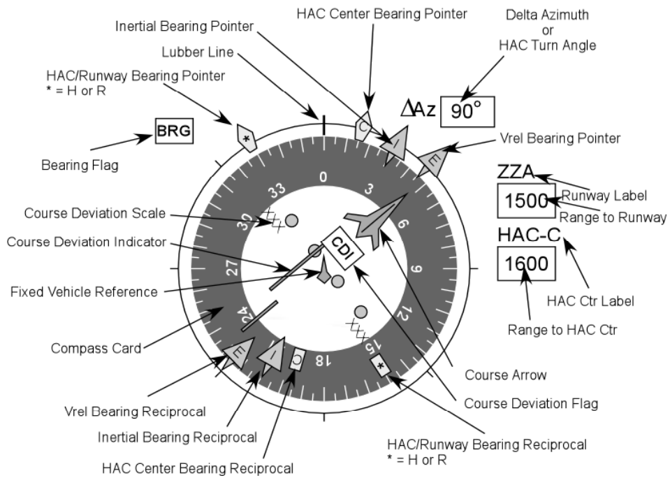
Figure 3-7. Horizontal Situation Indicator (HSI) and A/E PFD (for GSI)
