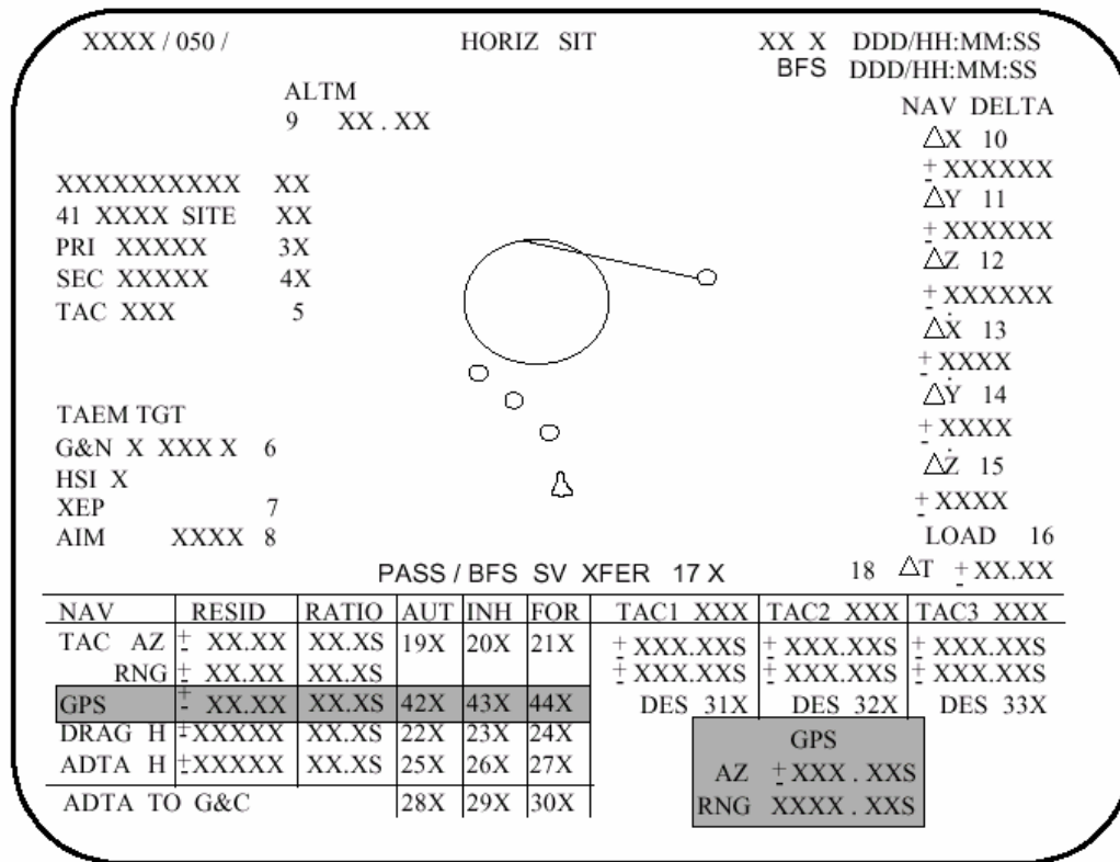
Figure 1-10. BFS single-string GPS SPEC 50 horizontal situation display
