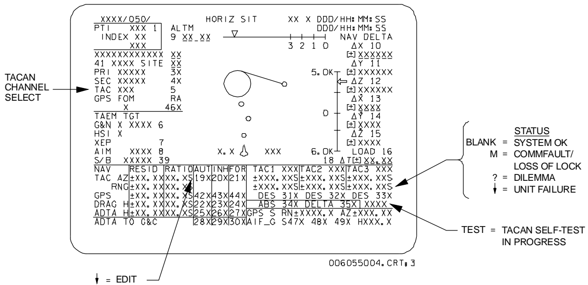
Figure 2-13. PASS GNC HORIZ SIT display
