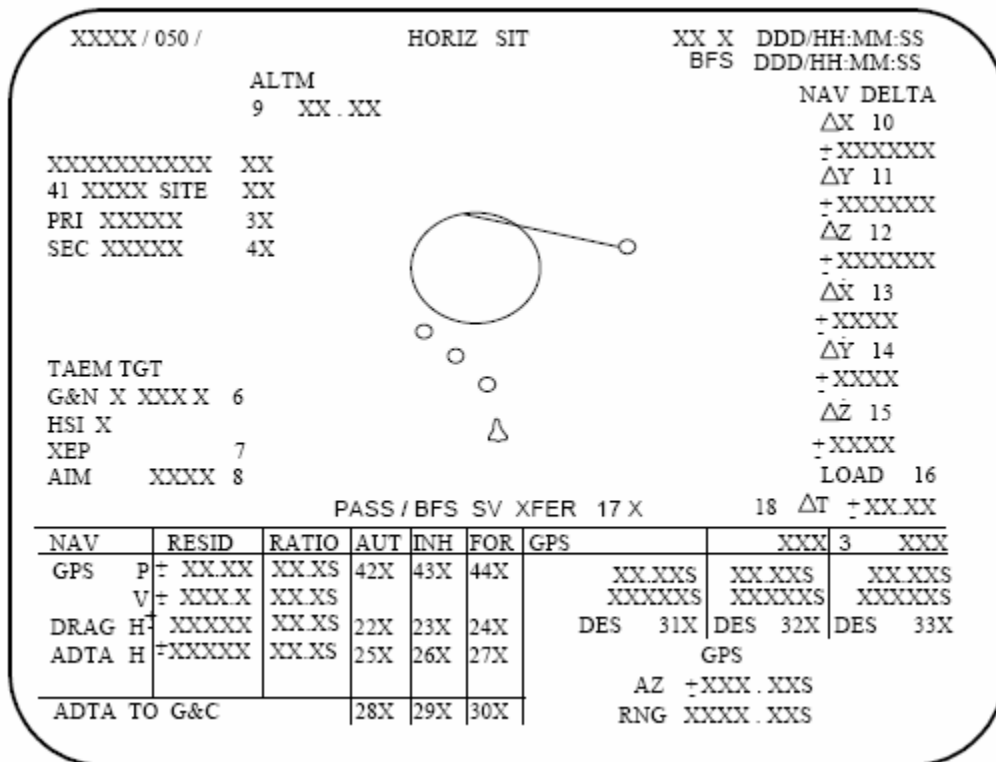
Figure 1-11. BFS three-string GPS SPEC 50 horizontal situation display
