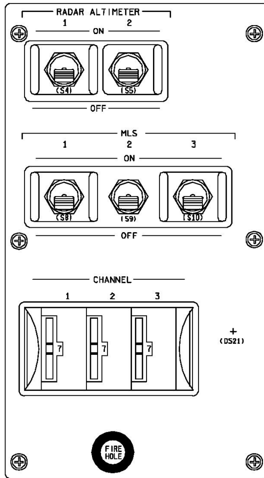
Figure 4-3. RA power switches on Panel O8
