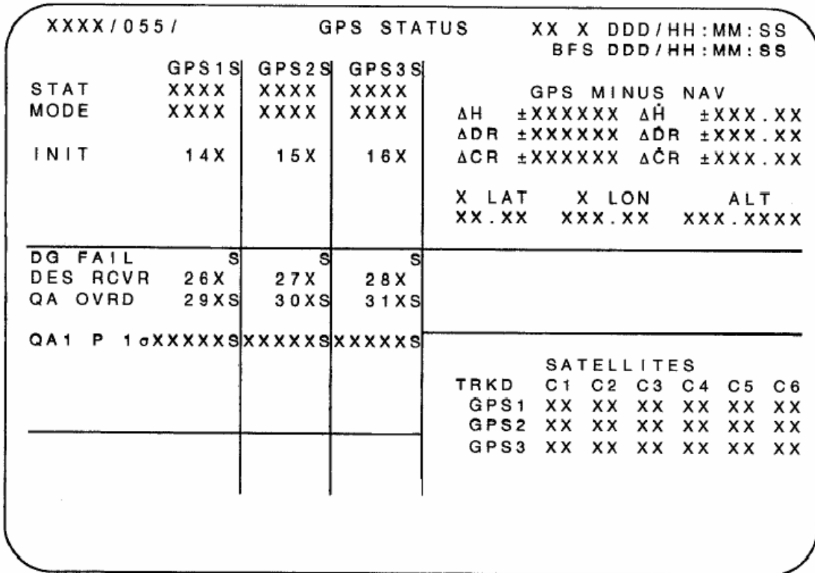
Figure 1-12. BFS SPEC 55 GPS STATUS display
