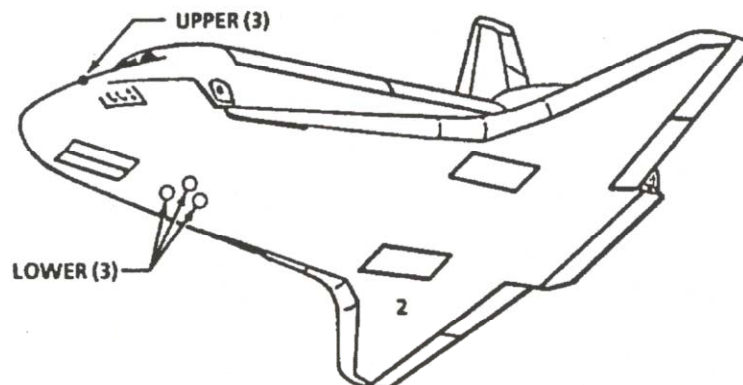
Figure 2-5. Orbiter TACAN antenna locations
