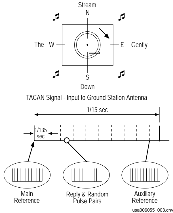
Figure 2-2. Rotating omnidirectional signal with fixed reference
