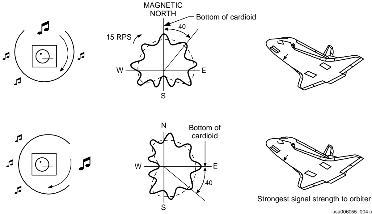
Figure 2-3. Rotating antenna makes signal directionally sensitive
