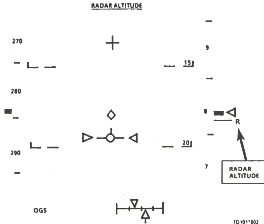
Figure 4-8. HUD display with radar altimeter
