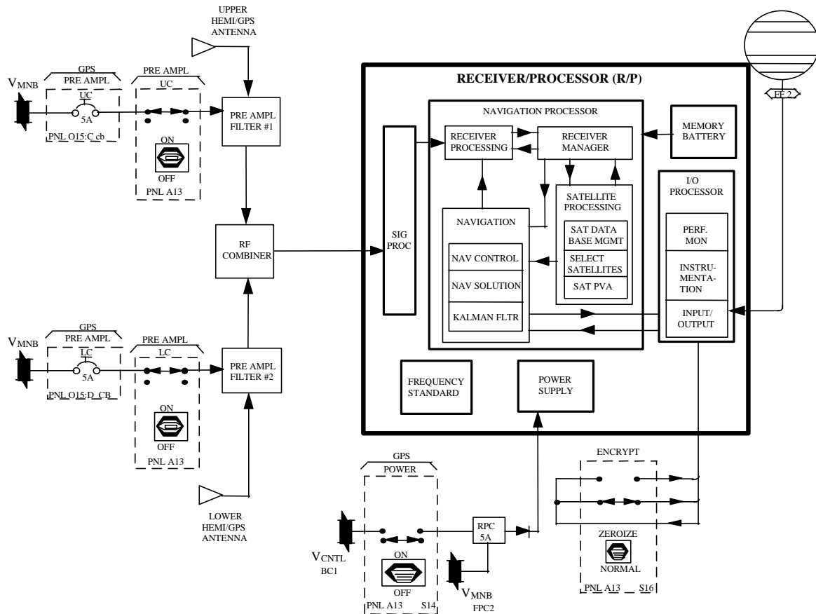
Figure 1-4. Single-string GPS switch configuration for OV-104
