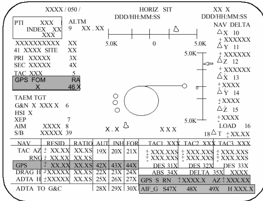
Figure 1-6. Single-string GPS SPEC 50 horizontal situation display
