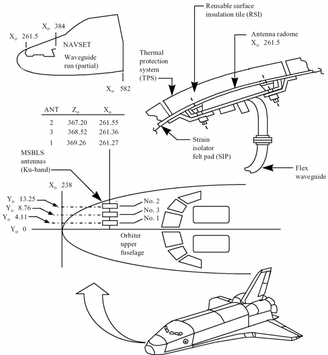
Figure 3-4. MLS antenna locations on orbiter
