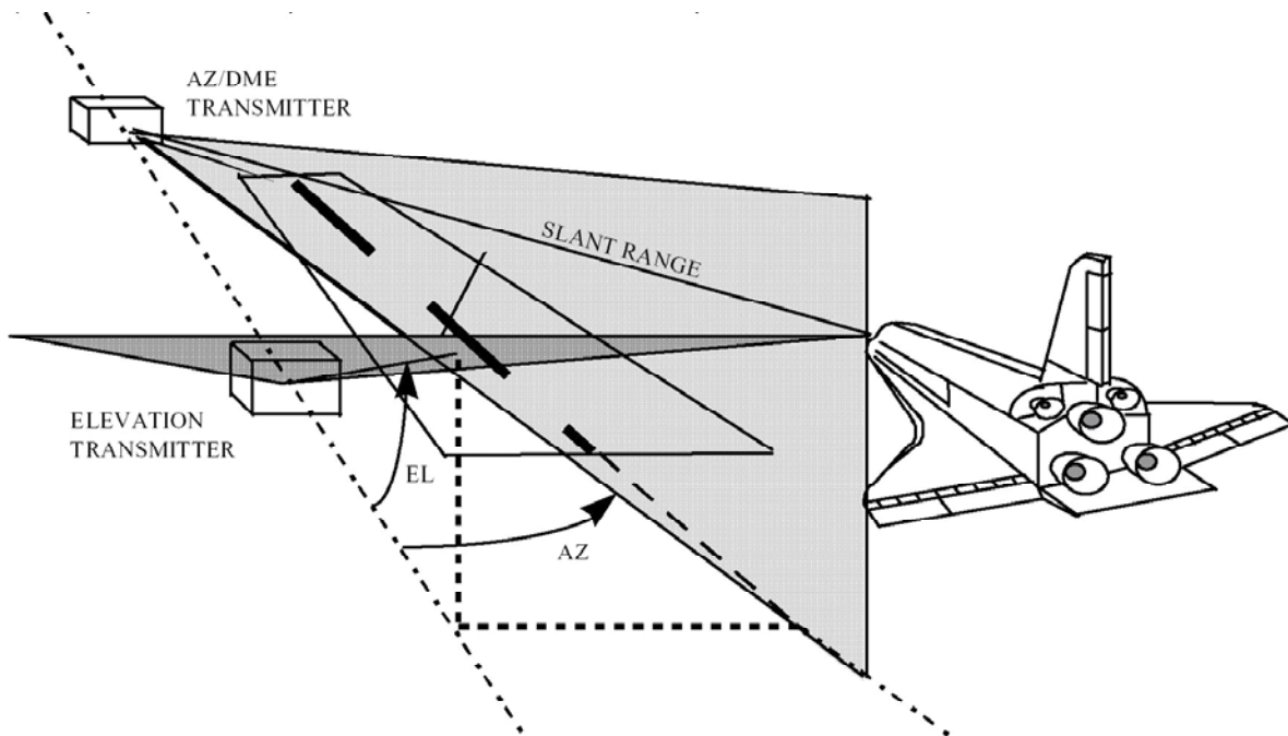
Figure 3-1. MLS beams and measurement geometry
