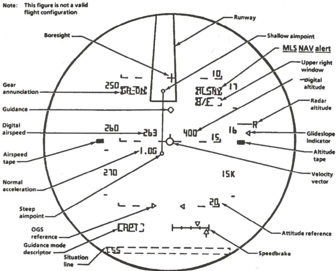
Figure 3-9. HUD display format 1 (approach and landing)
