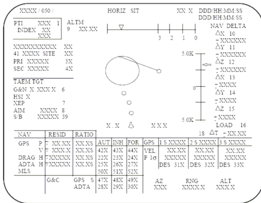
Figure 1-7. Three-string GPS SPEC 50 horizontal situation display
