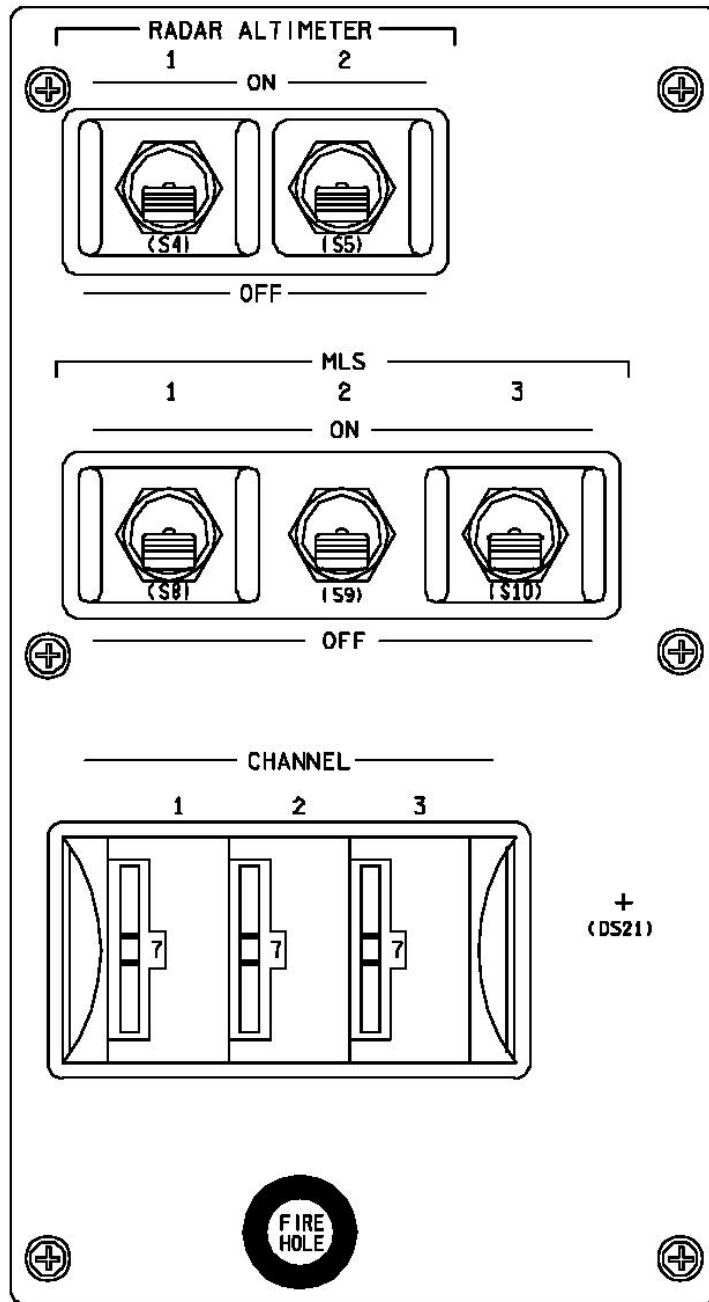
Figure 3-6. MLS power switches and channel thumbwheels on Panel O8
