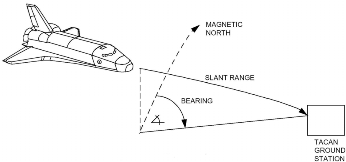
Figure 2-1. TACAN output data
