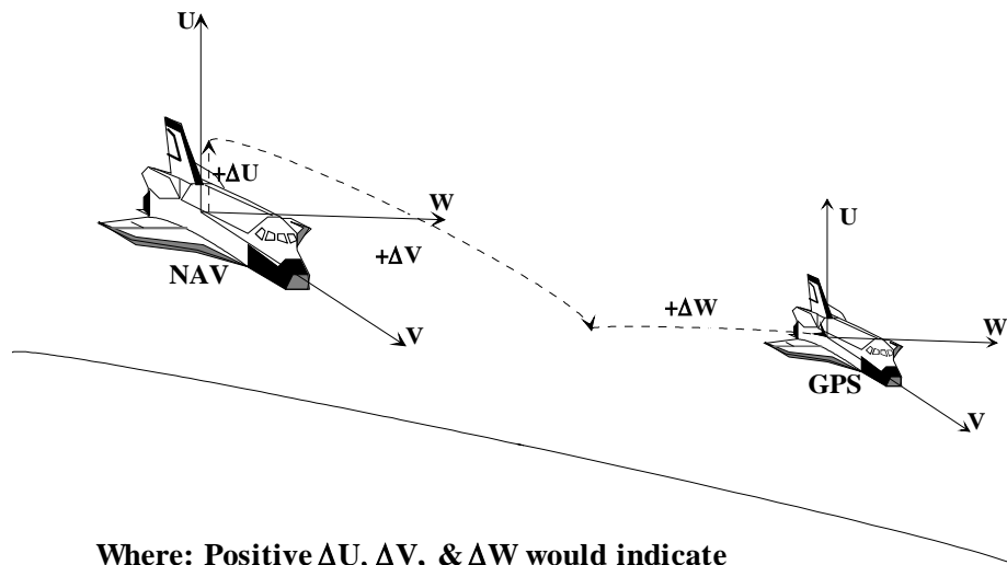
Figure 1-9. GPS minus NAV illustration
