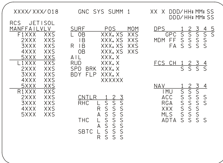
Figure 3-10. GNC system summary 1 display
