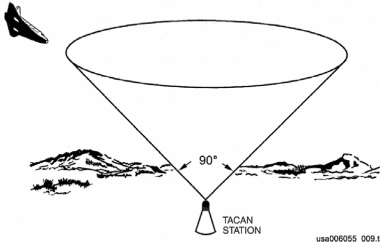
Figure 2-19. Bearing cone of confusion
