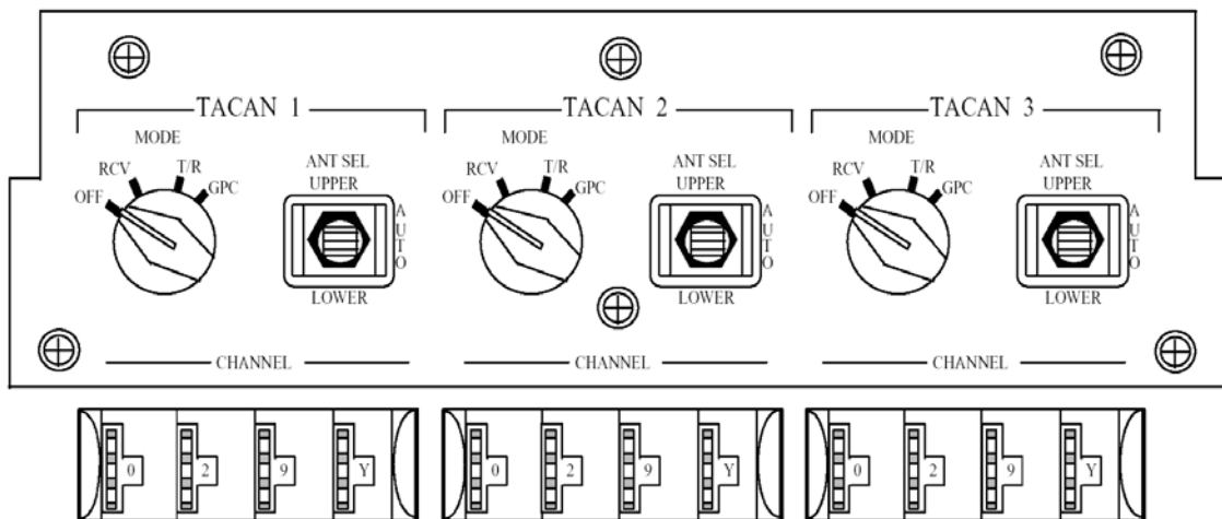
Figure 2-7. TACAN system controls
