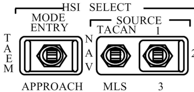
Figure 3-8. HSI select switches on Panels F6 and F8
