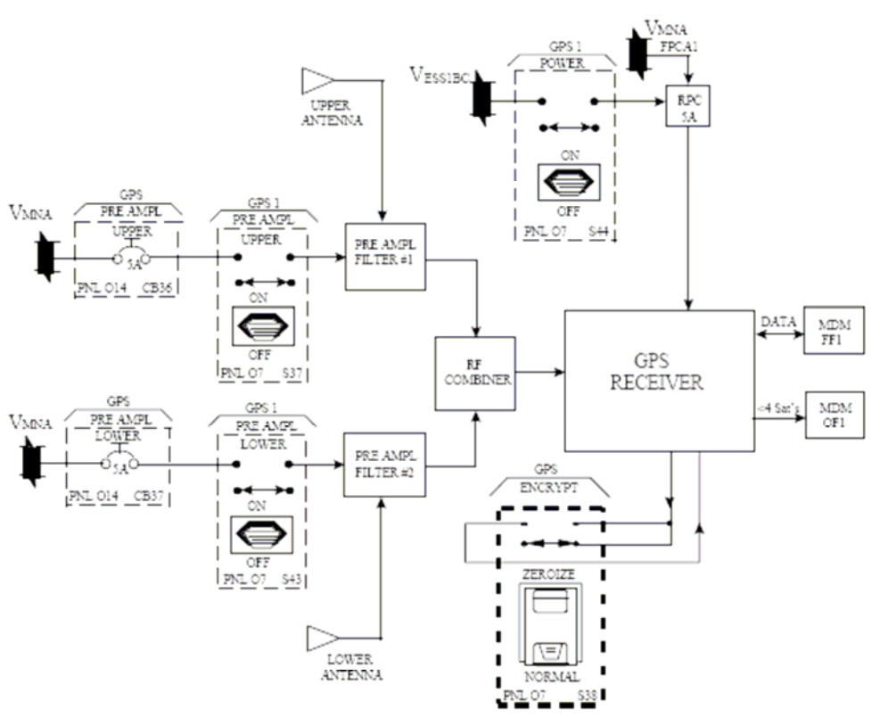
Figure 1-5. Three-string GPS switch configuration for OV-105
