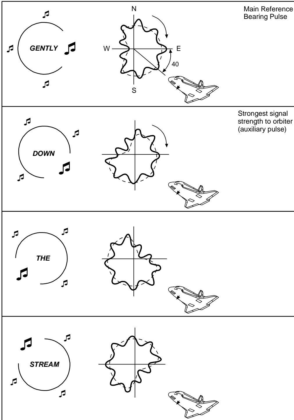
Figure 2-4. Bearing determination
